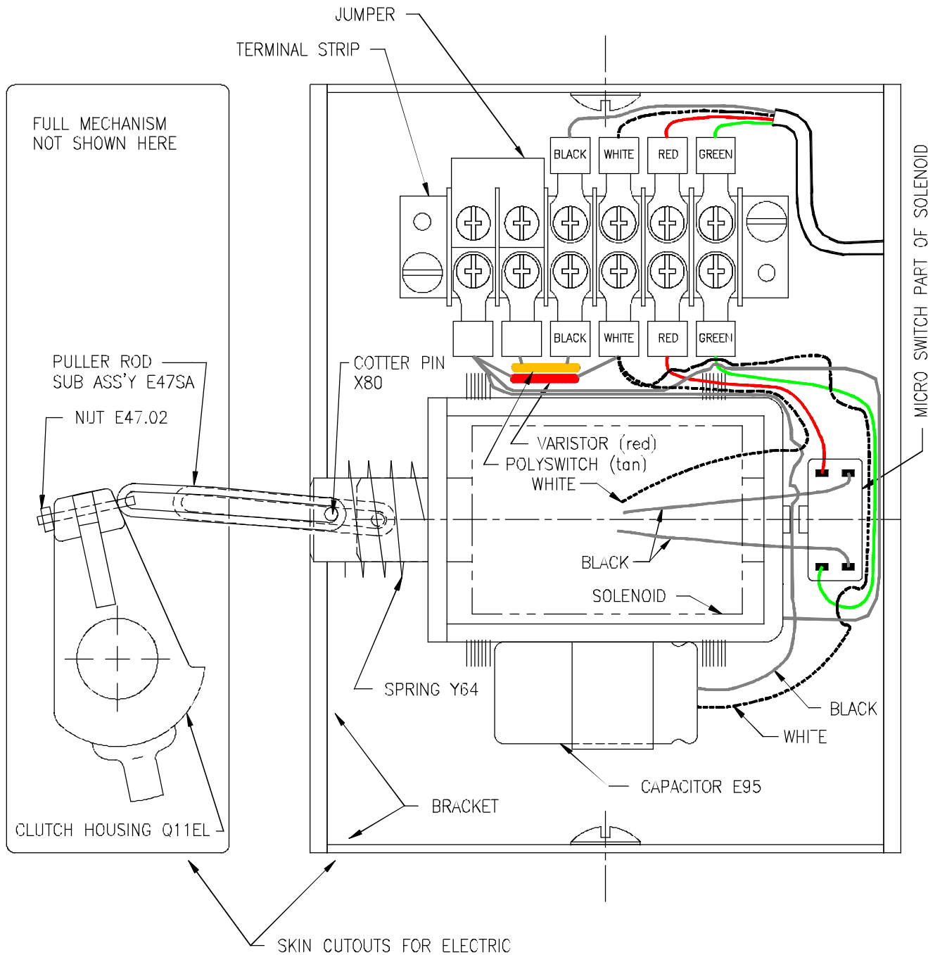
CUTAWAY VIEW - "E-UNL" MECH. (E19SA-EUN) - LH OR LR
